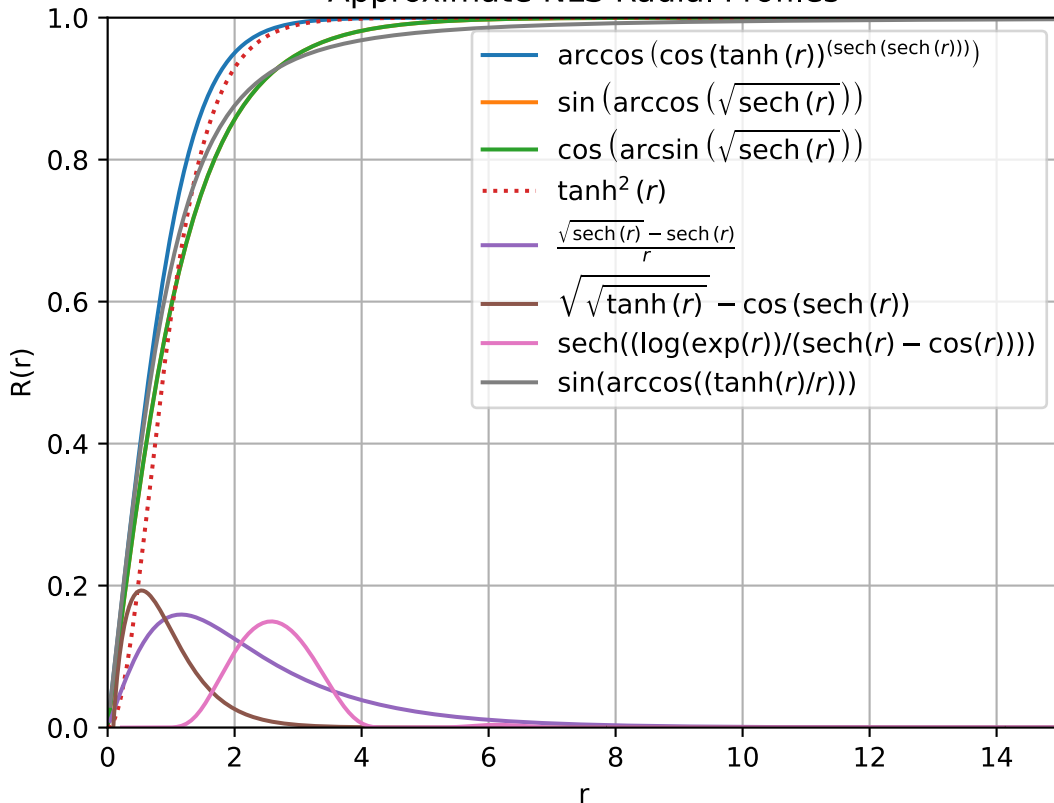
Approximate NLS Radial Profiles
