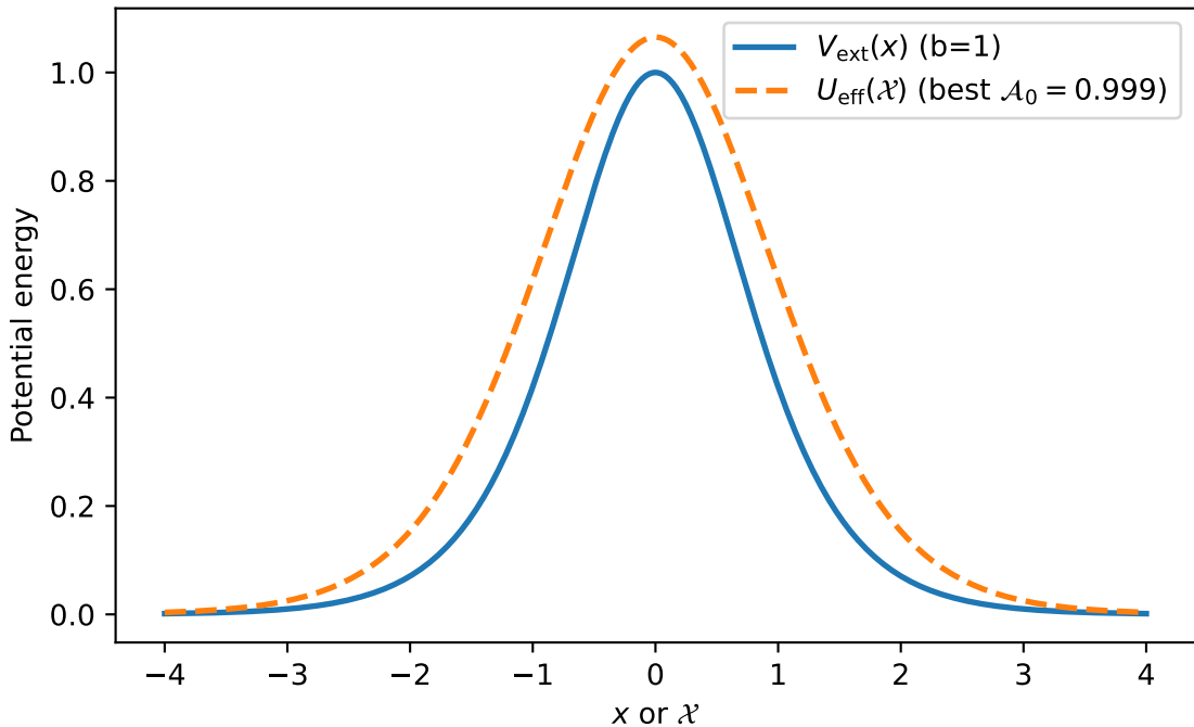
Best fit of U_{\text{eff}} to V_{\text{ext}} ( A = b = 1 , \Omega = 0.2 )
