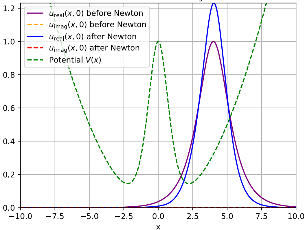
V(x) , u_{\text{real}}(x, 0) and u_{\text{imag}}(x, 0)
