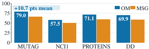
Accuracy (%) on four TU benchmarks
