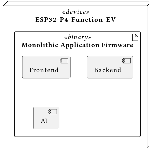
Figure 4: Deployment View
