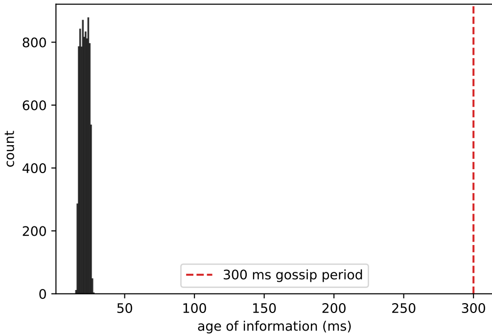
Data-plane Aol (gossip staleness), N=8
