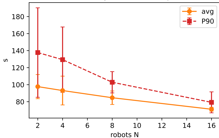
Task latency (create->complete)
