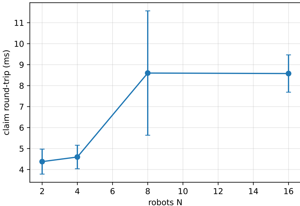
Claim overhead T_{claim} vs fleet size
