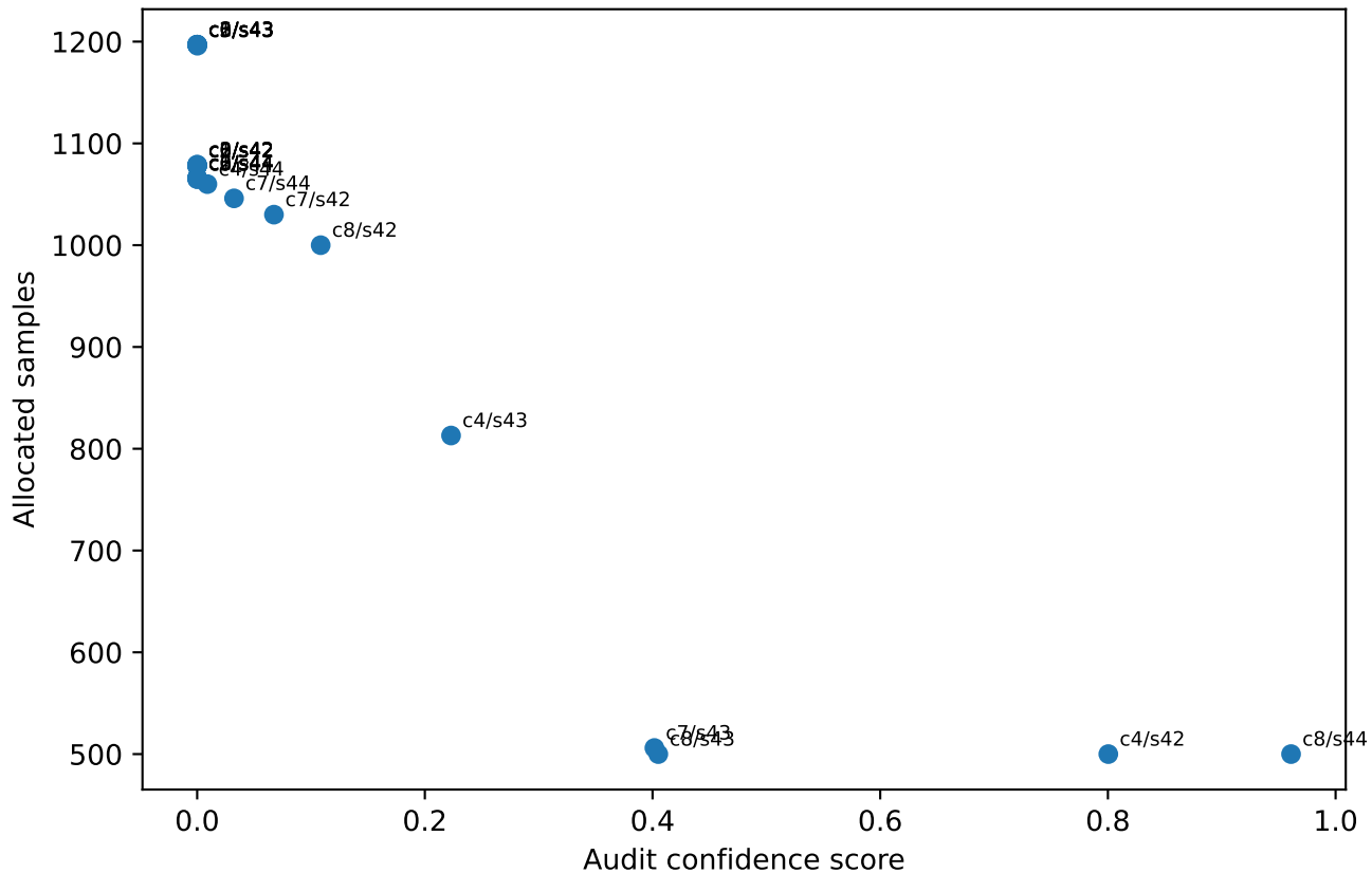
Class-repair allocation versus audit confidence
