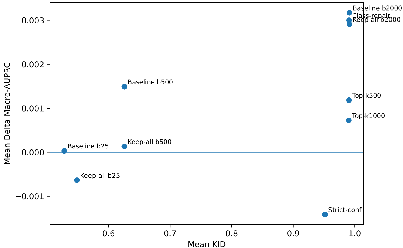
Mean KID vs Mean Delta Macro-AUPRC
