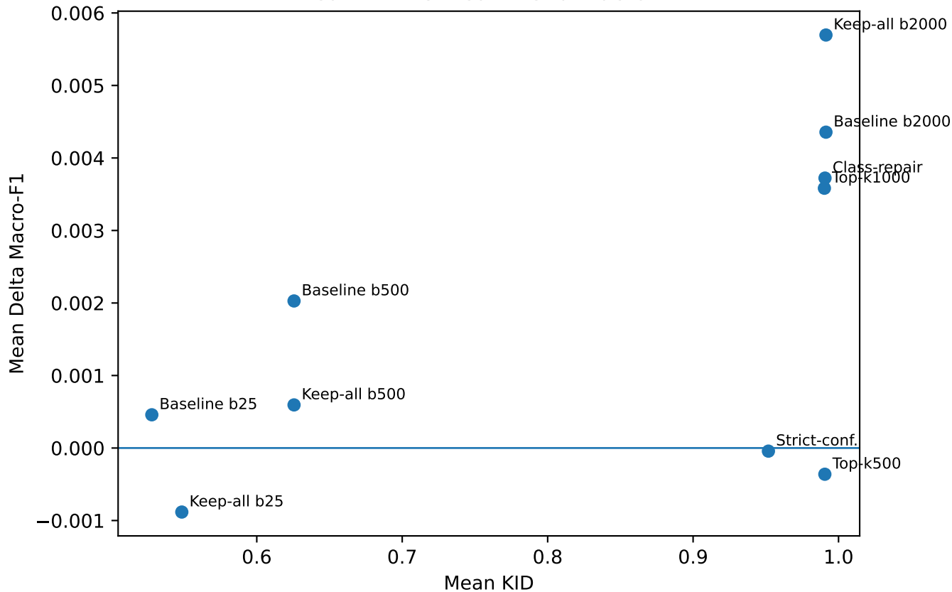
Mean KID vs Mean Delta Macro-F1
