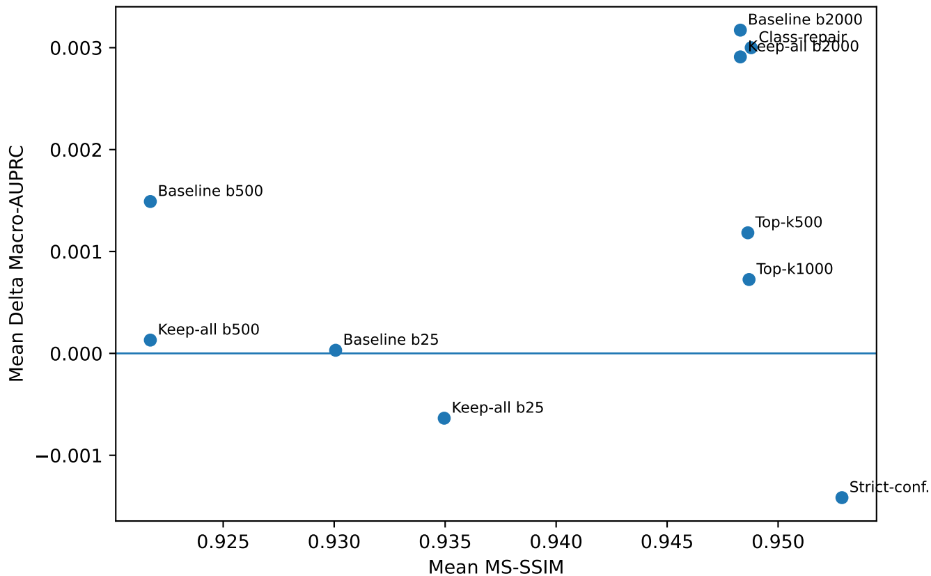
Mean MS-SSIM vs Mean Delta Macro-AUPRC
