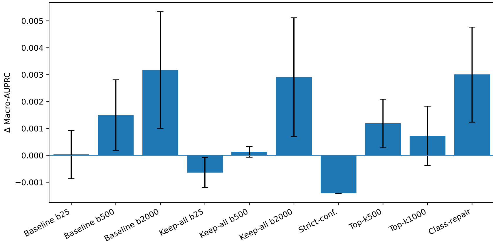
Policy effect on Macro-AUPRC
