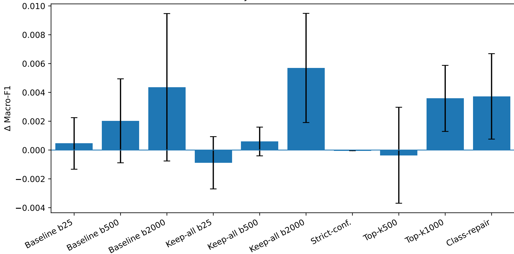
Policy effect on Macro-F1
