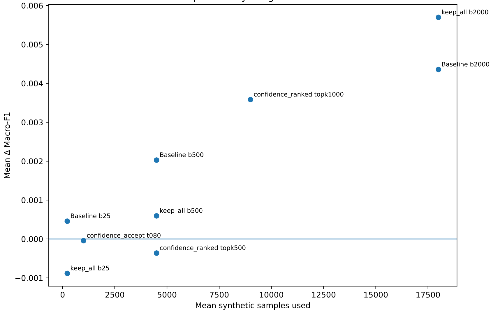
Paper 4 utility-budget tradeoff
