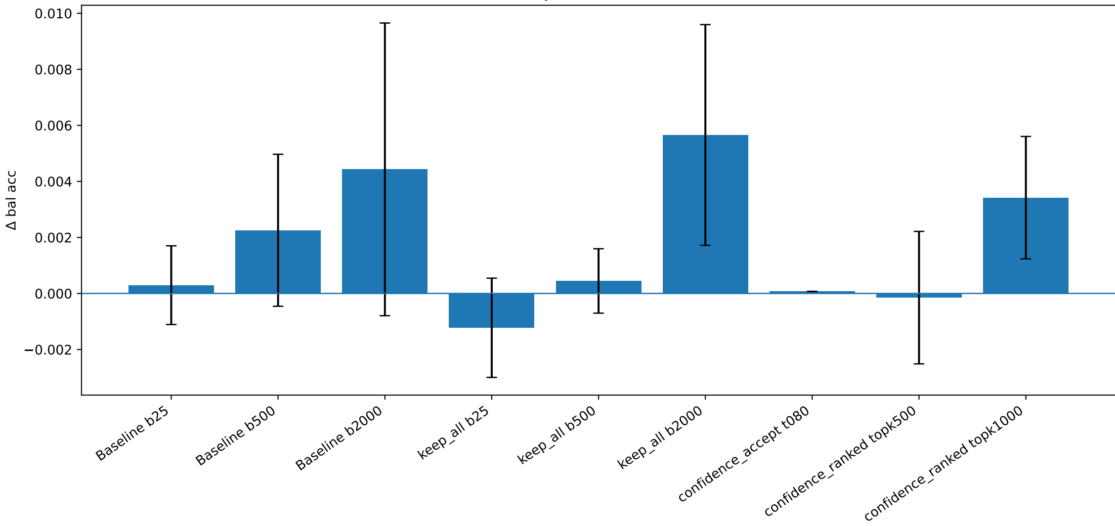
Policy effect on bal acc
