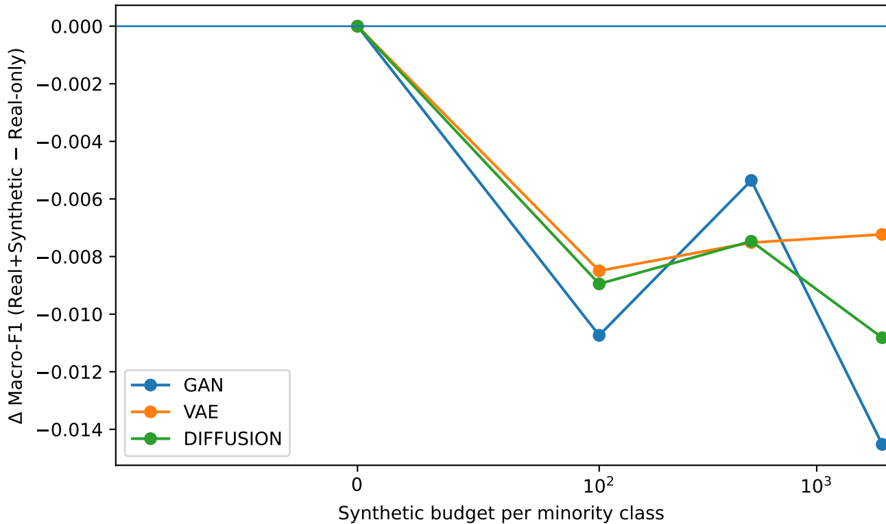
Minority-heavy c4/c7 minority-only augmentation
