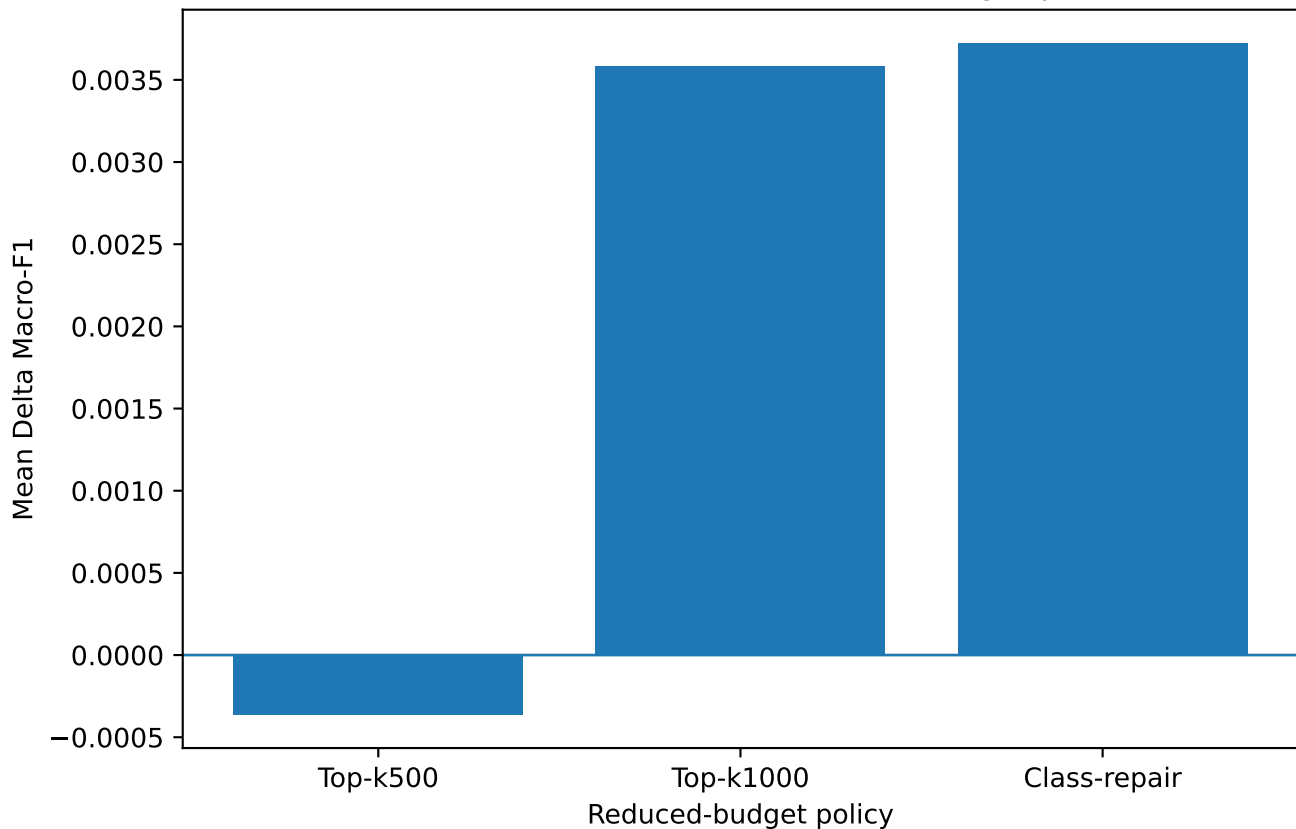
Mean Delta Macro-F1 under reduced-budget policies
