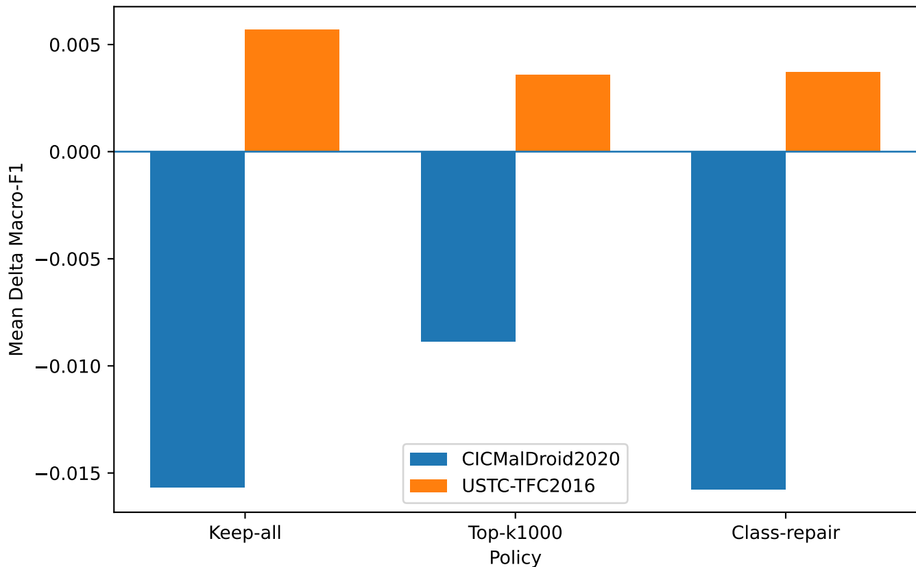
Mean Delta Macro-F1 across datasets
