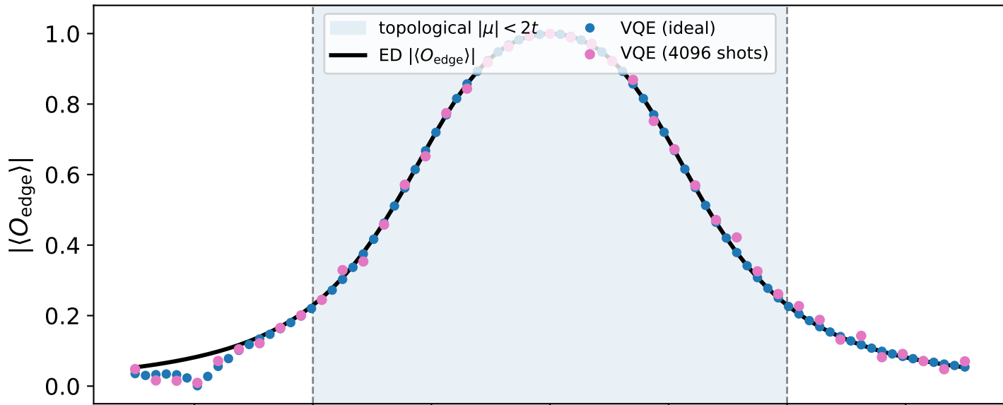
Week 7: VQE-prepared edge-string sweep ( L=4 , t=1 , \Delta=1 )
