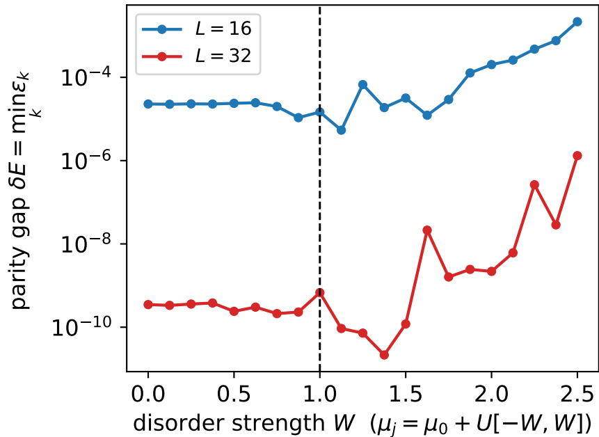
Parity gap: protected until W \sim \Delta
