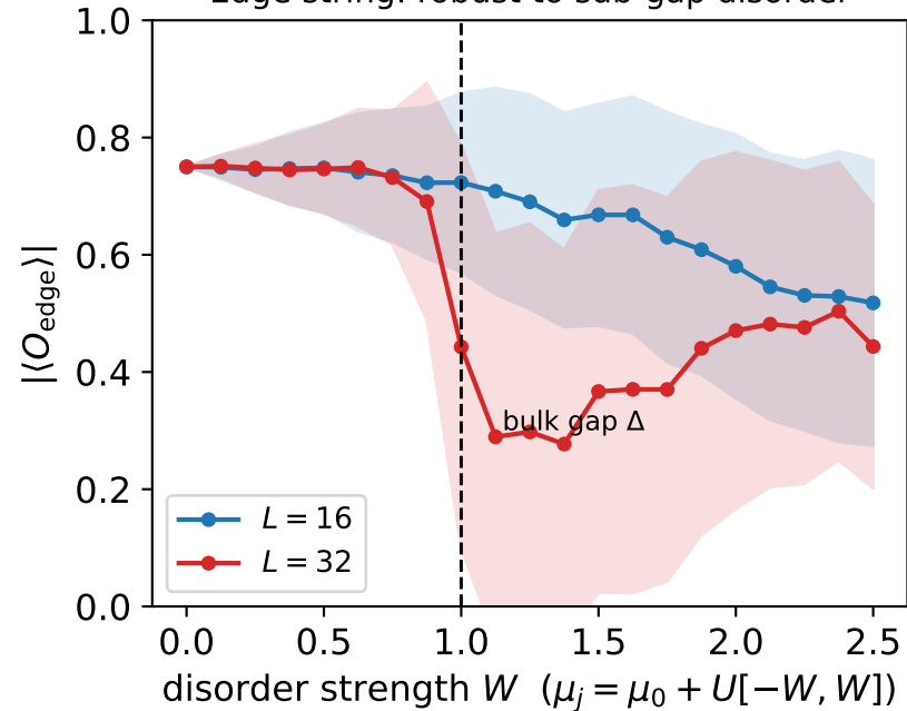
Edge string: robust to sub-gap disorder
