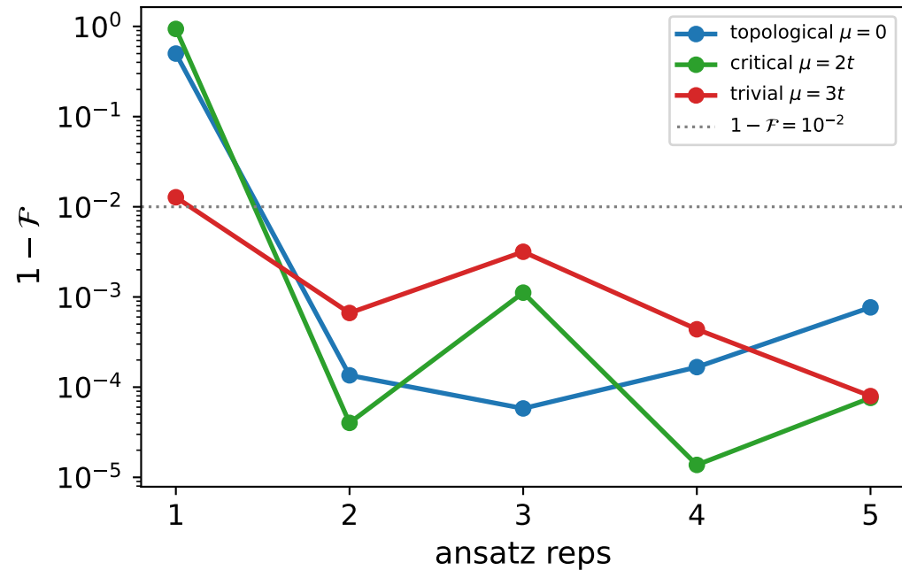
Subspace infidelity vs depth
