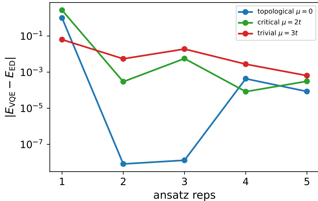
Energy error vs depth
