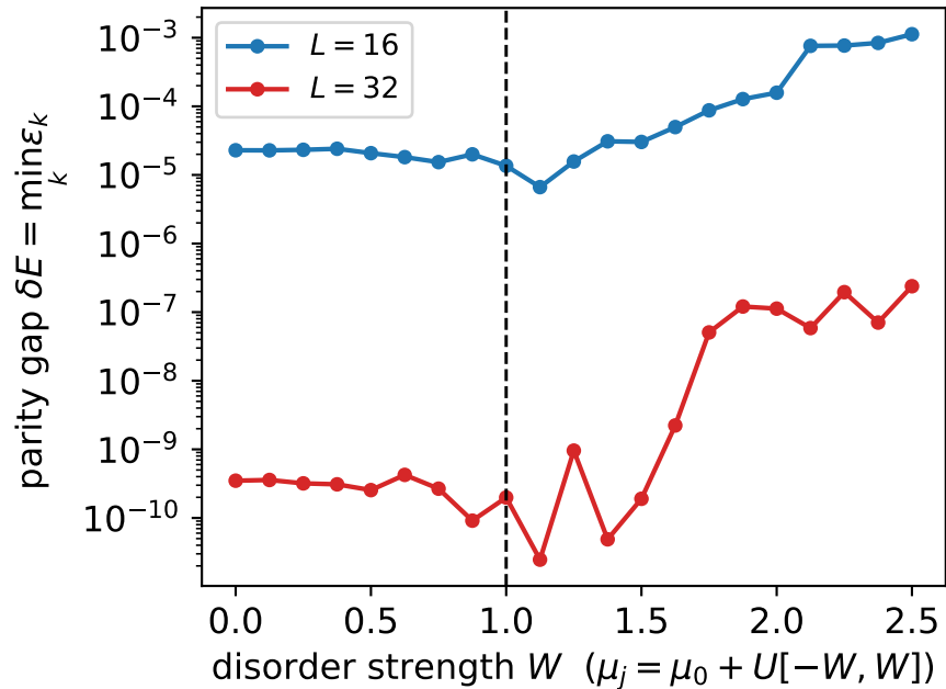
Parity gap: protected until W \sim \Delta
