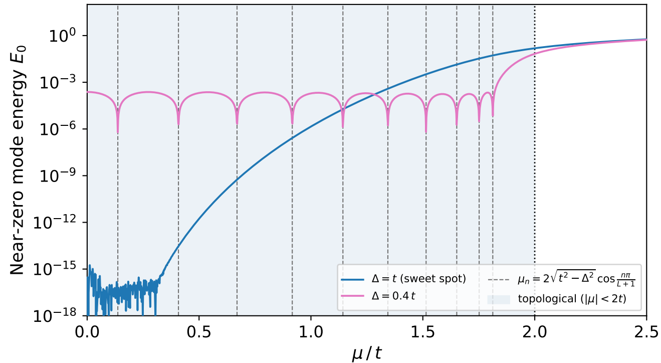
Exact zero-energy (Majorana) lines ( L = 20 , OBC)
