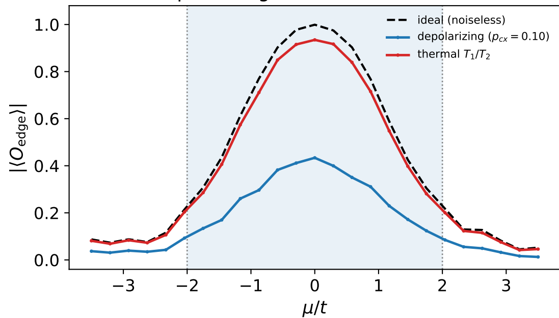
Depolarizing vs thermal relaxation
