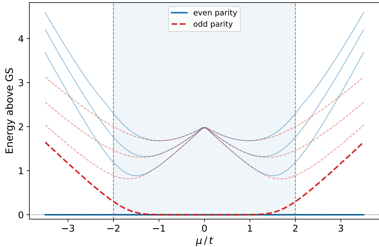
Many-body qubit spectrum ( L = 10 )
