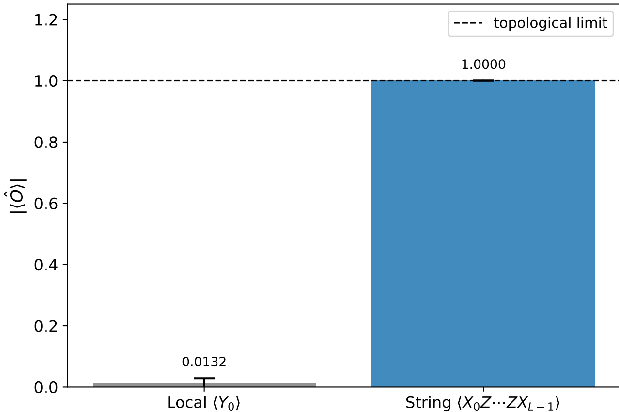
Majorana signatures at \mu = 0 ( L = 4 )
