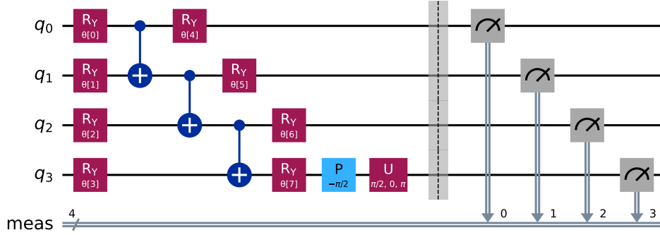
Figure 3: The measurement circuit for the non-local String Order Parameter (SOP).
