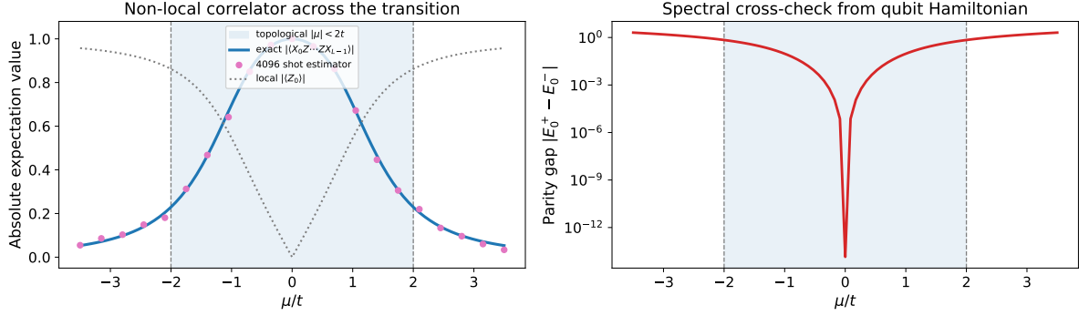
Figure 1: Week 6 phase sweep for L = 4 , t = \Delta = 1 . The left panel shows the non-local edge-string correlator and a finite-shot estimator. The right panel shows the parity-gap cross-check.
