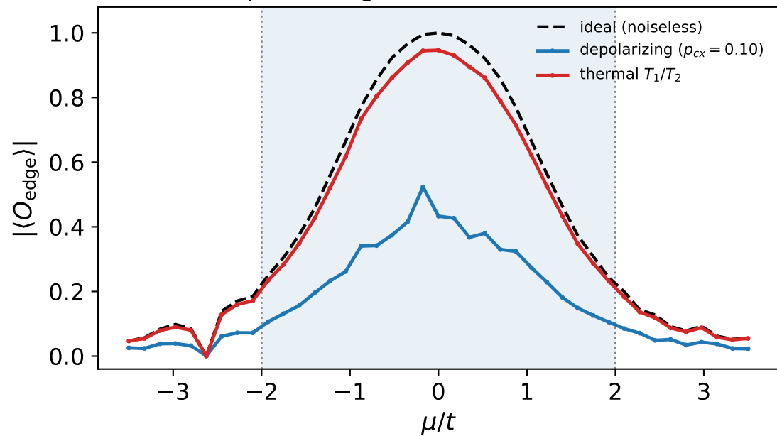
Depolarizing vs thermal relaxation
