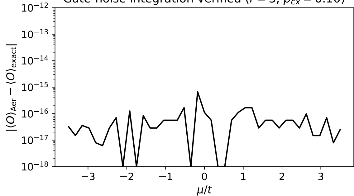
Gate-noise integration verified ( r = 3 , p_{CX} = 0.10 )
