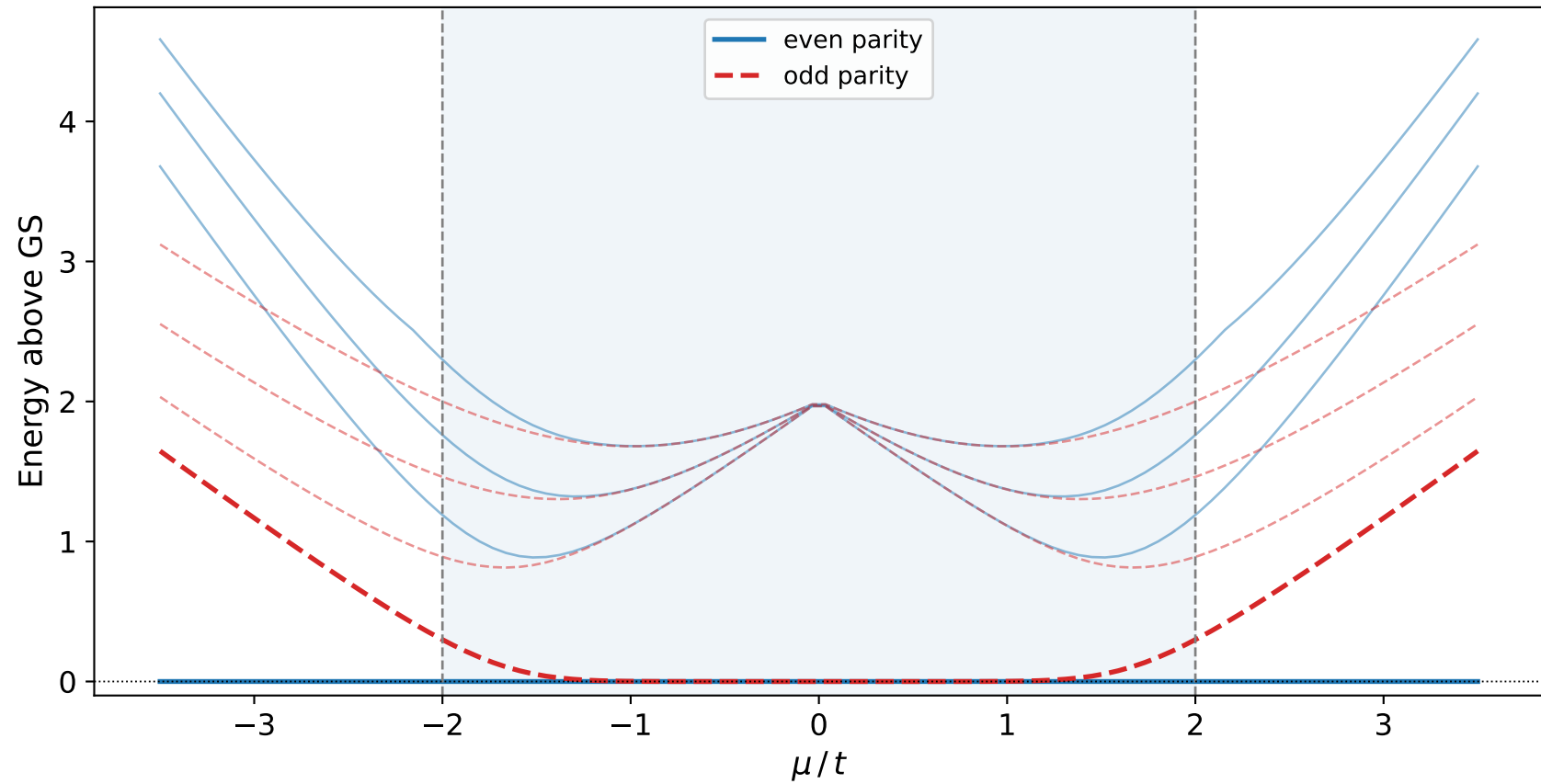
Many-body qubit spectrum ( L = 10 , t = \Delta = 1 , OBC)
