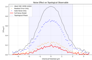
(c) ReadoutError:0.25, GateError:0.15
