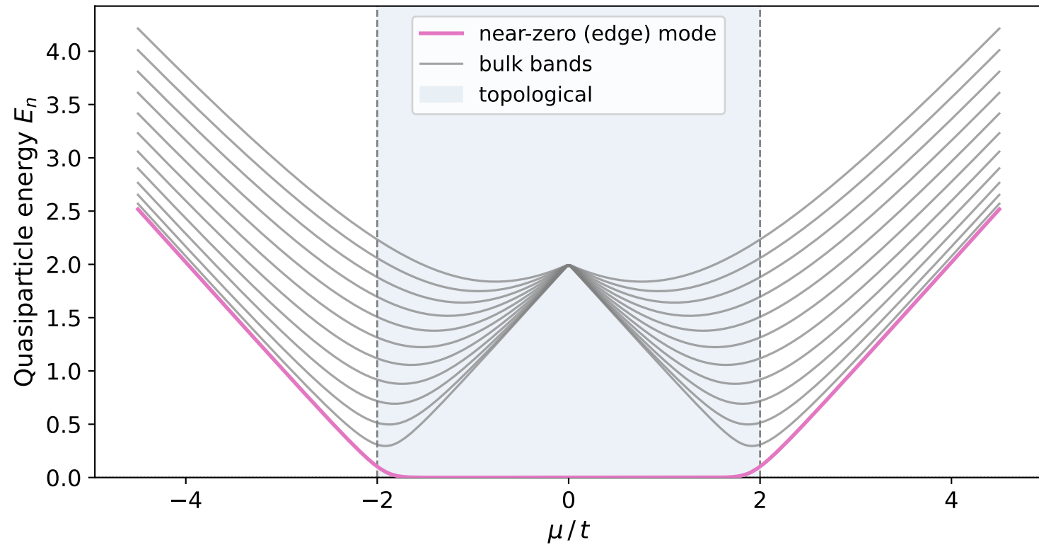
Finite-size BdG spectrum ( L = 30 , OBC, t = \Delta = 1 )
