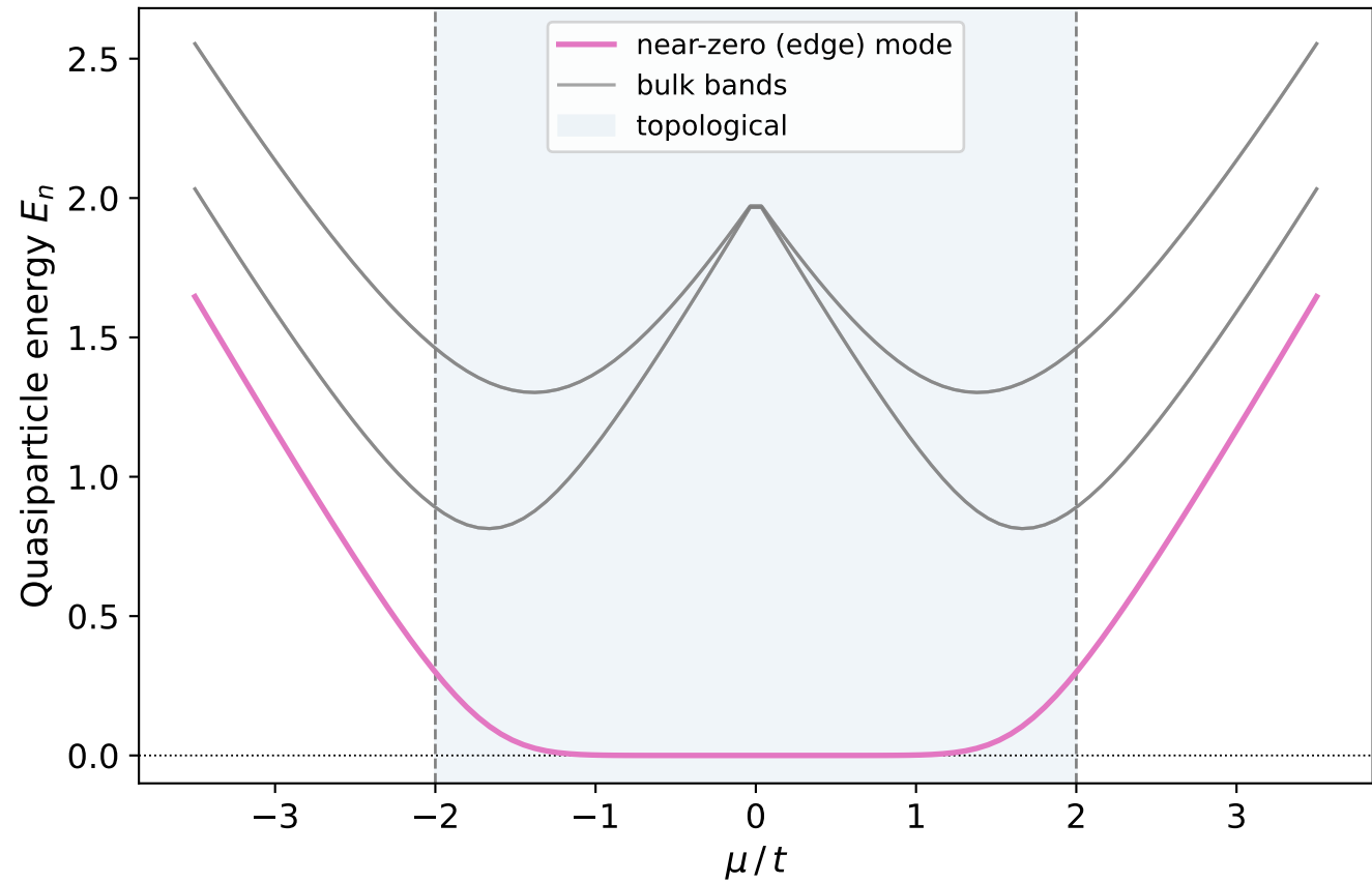
Finite-size BdG spectrum ( L = 10 )
