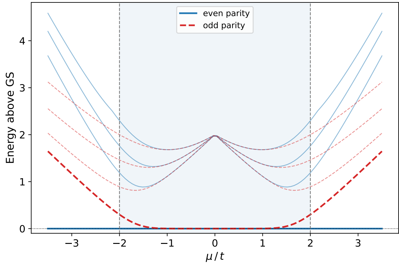
Many-body qubit spectrum ( L = 10 )
