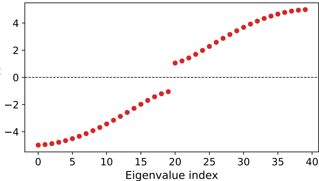
Trivial \mu = -3t
