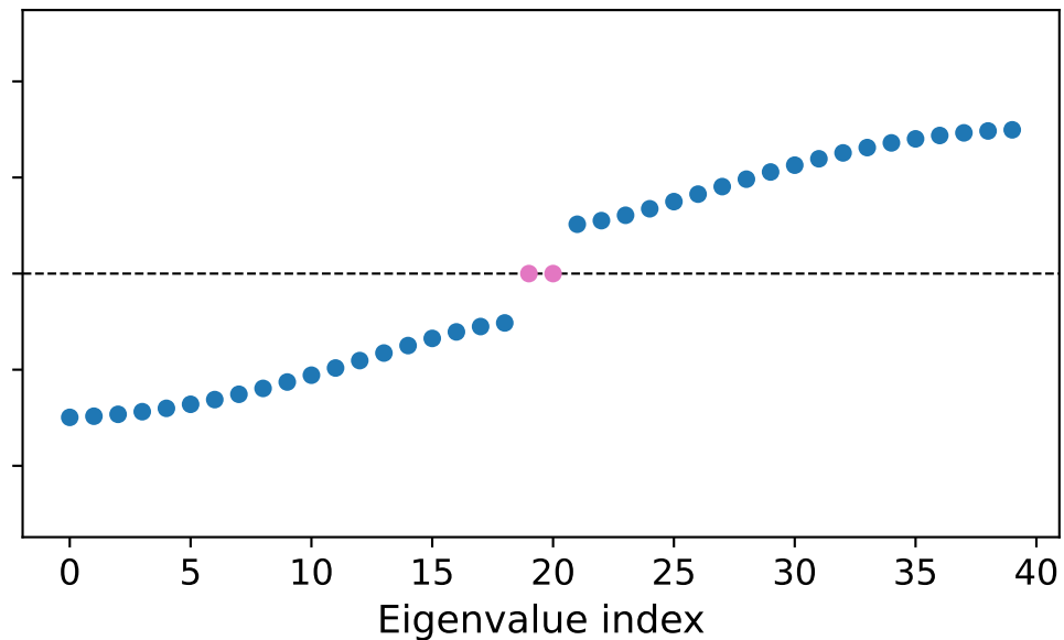
Topological \mu = -t
