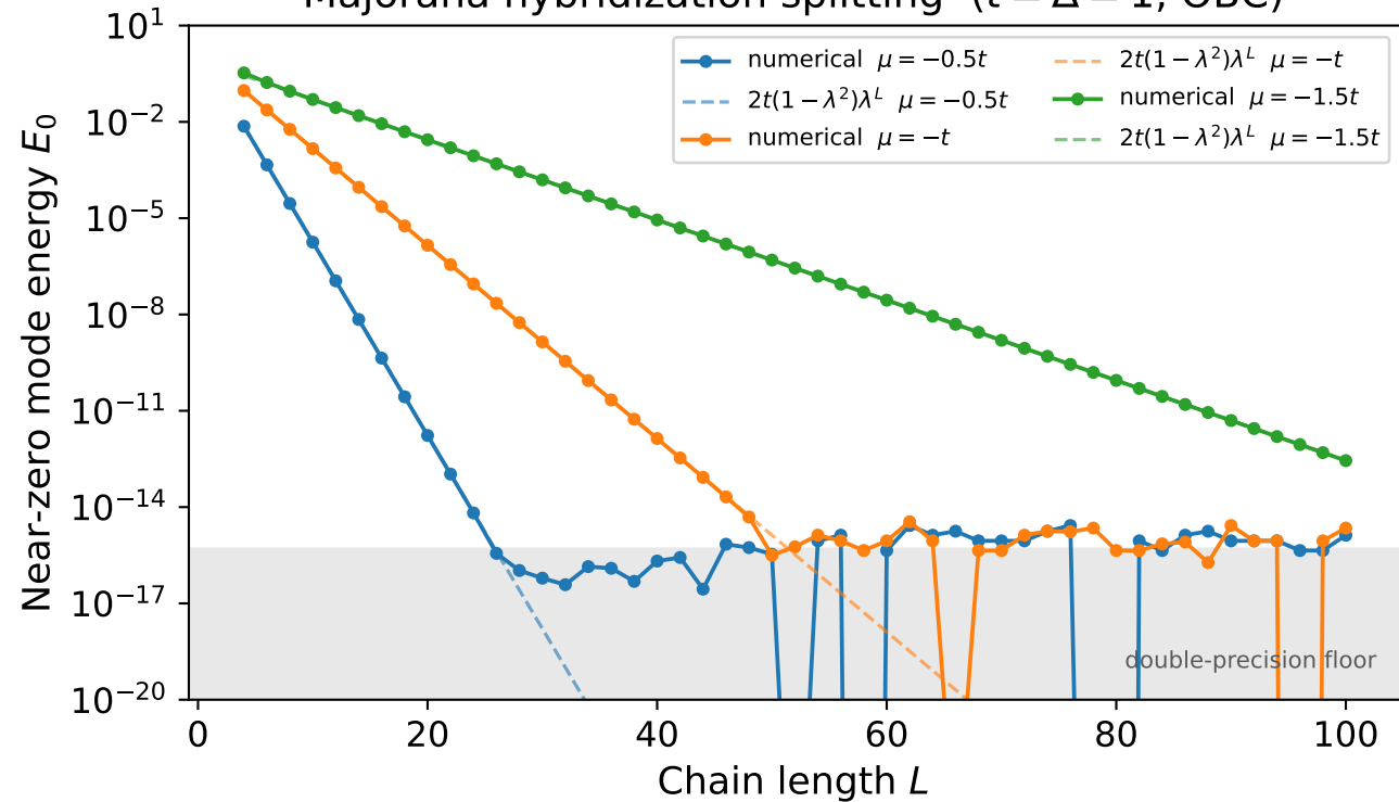
Majorana hybridization splitting ( t = \Delta = 1 , OBC)
