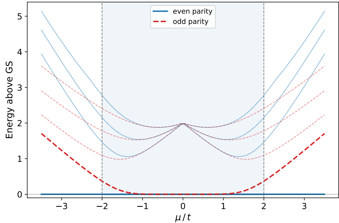
Many-body qubit spectrum ( L = 8 )
