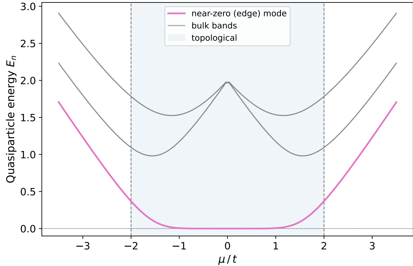
Finite-size BdG spectrum ( L = 8 )
