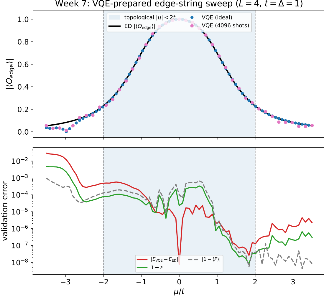
Figure 1: Week 7 VQE-prepared sweep for L = 4, t = \Delta = 1 . Top: the edge string |\langle O_{\text{edge}} \rangle| from parity-constrained VQE, both ideal and shot-based, plotted against the ED baseline. Bottom: per-point validation showing energy error, infidelity 1 - \mathcal{F} , and parity deviation |1 - \langle P \rangle| ; crosses mark points that required random-restart recovery.
