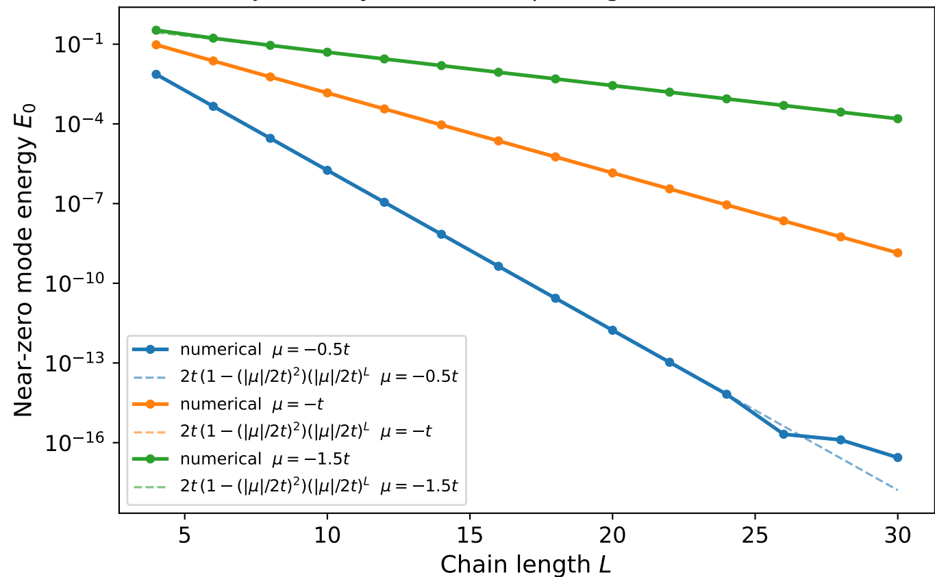
Majorana hybridization splitting ( t = \Delta = 1 , OBC)
