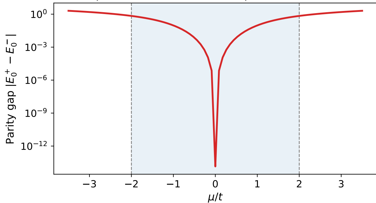
Spectral cross-check from qubit Hamiltonian
