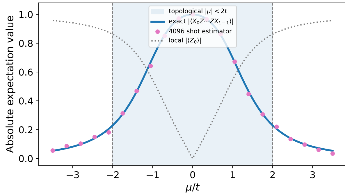
Non-local correlator across the transition
