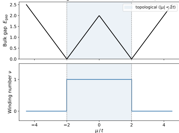
Phase diagram of the Kitaev chain ( t = \Delta = 1 )
