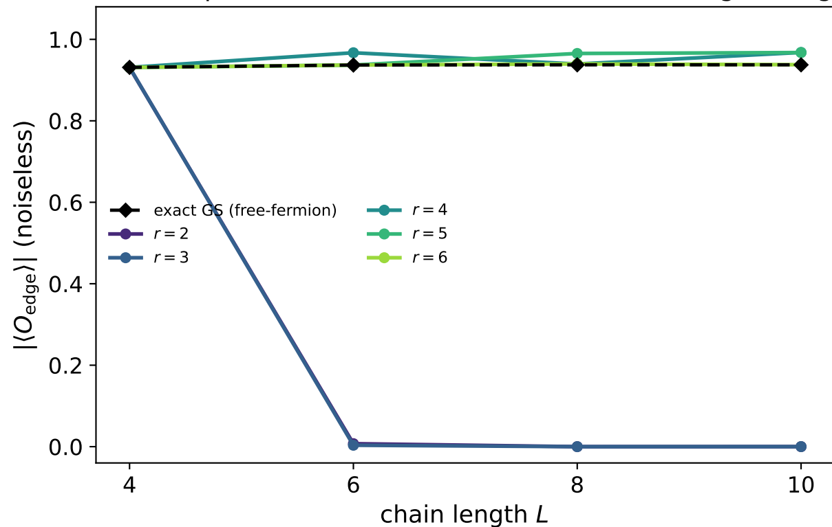
Fixed depth: shallow circuits cannot build the edge string
