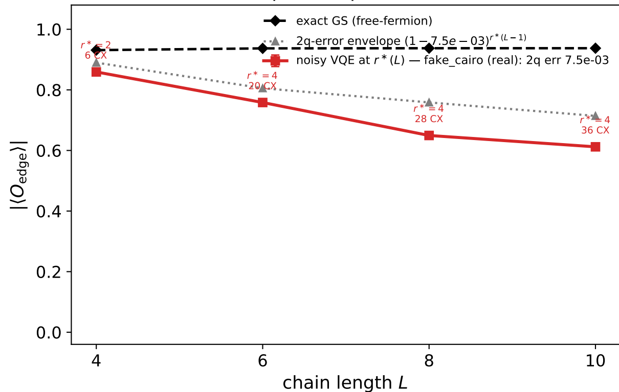
Minimal adequate depth: noise then wins
