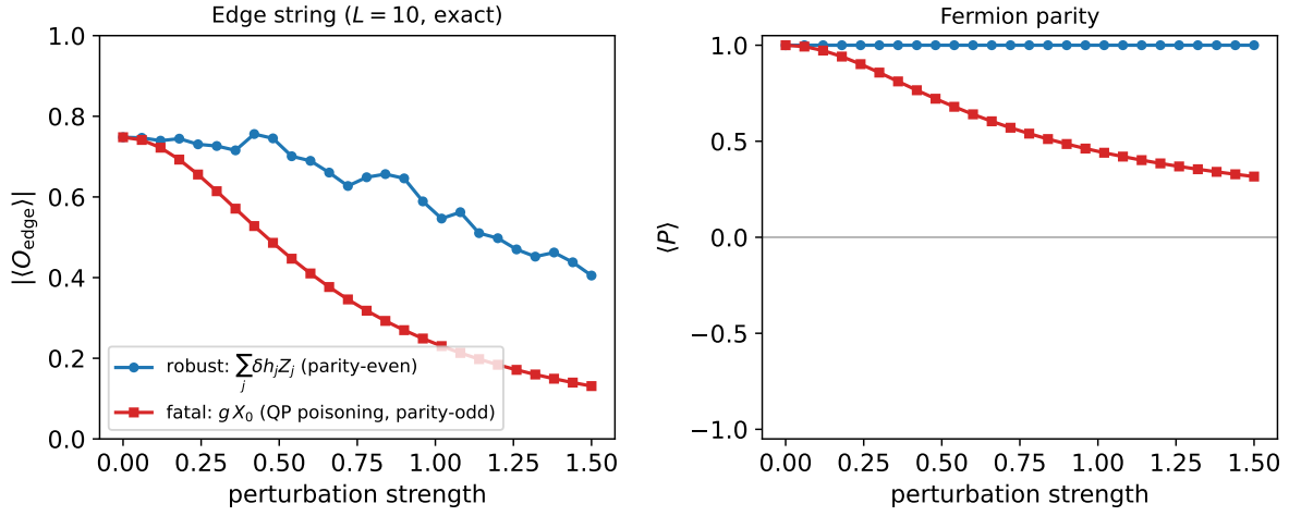
Figure 2: Robust vs fatal , same L , exact. Blue : parity-preserving \sum_j \delta h_j Z_j keeps \langle \hat{P} \rangle = +1 and the edge string near its topological value. Red : the parity-odd quasiparticle term g X_0 collapses both the parity and the edge string with no protective threshold. Topological protection is protection against local, parity-preserving, sub-gap noise only .
