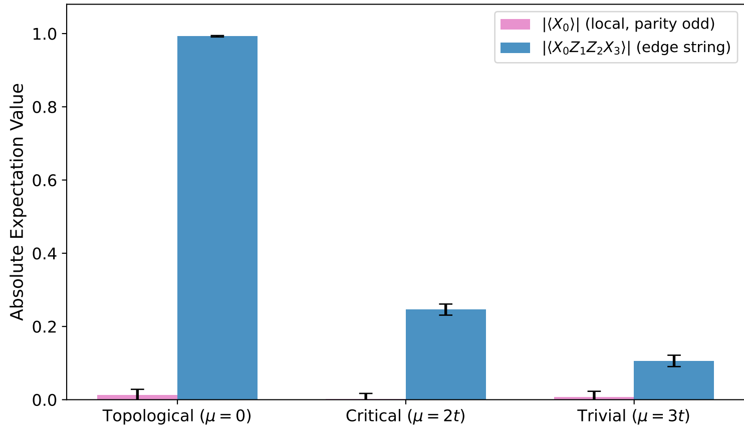
Shot-Based Edge-String Measurements via VQE ( L = 4 )
