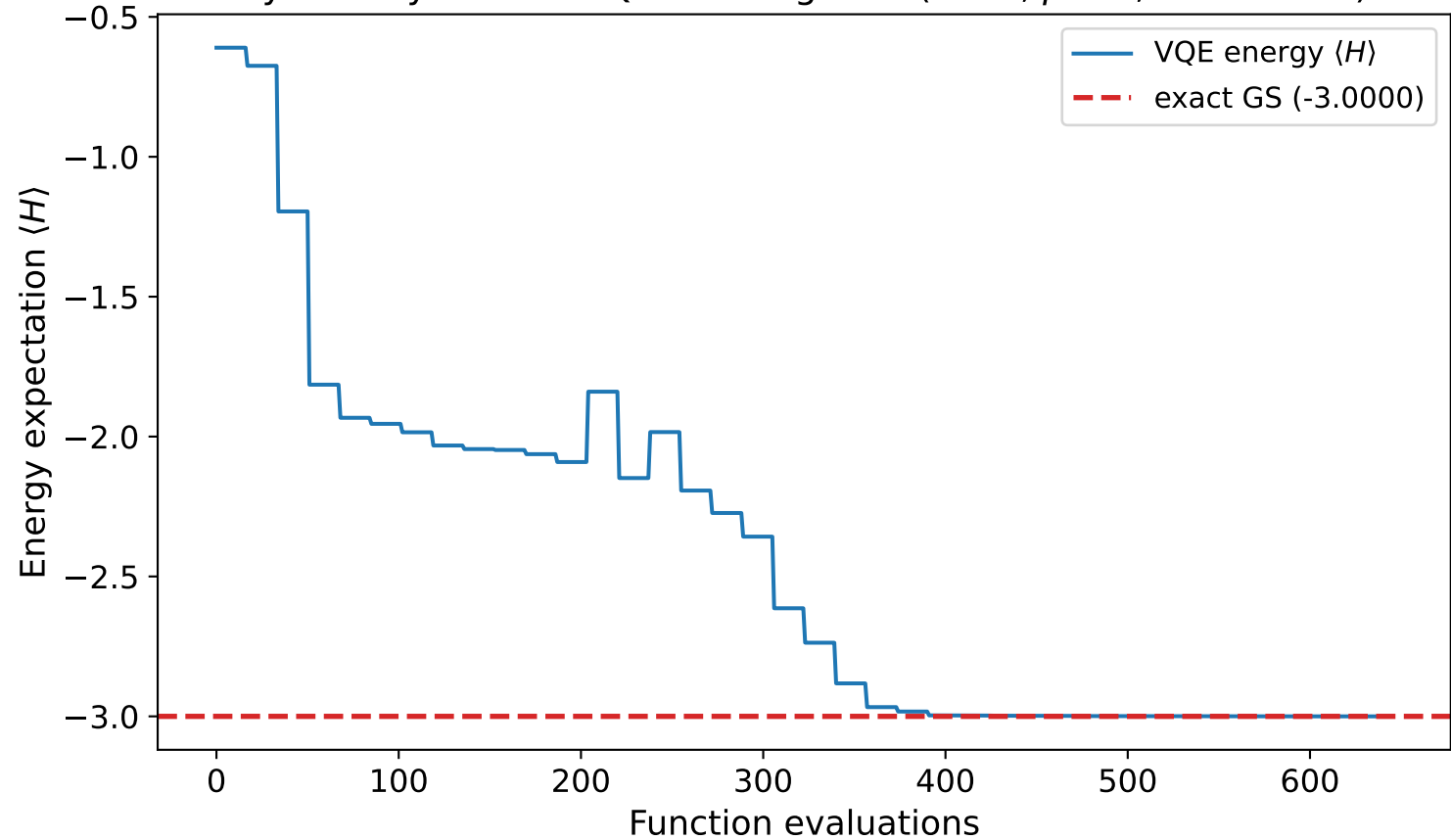
Symmetry-broken VQE convergence ( L = 4, \mu = 0, \mathcal{F} = 1.0000 )
