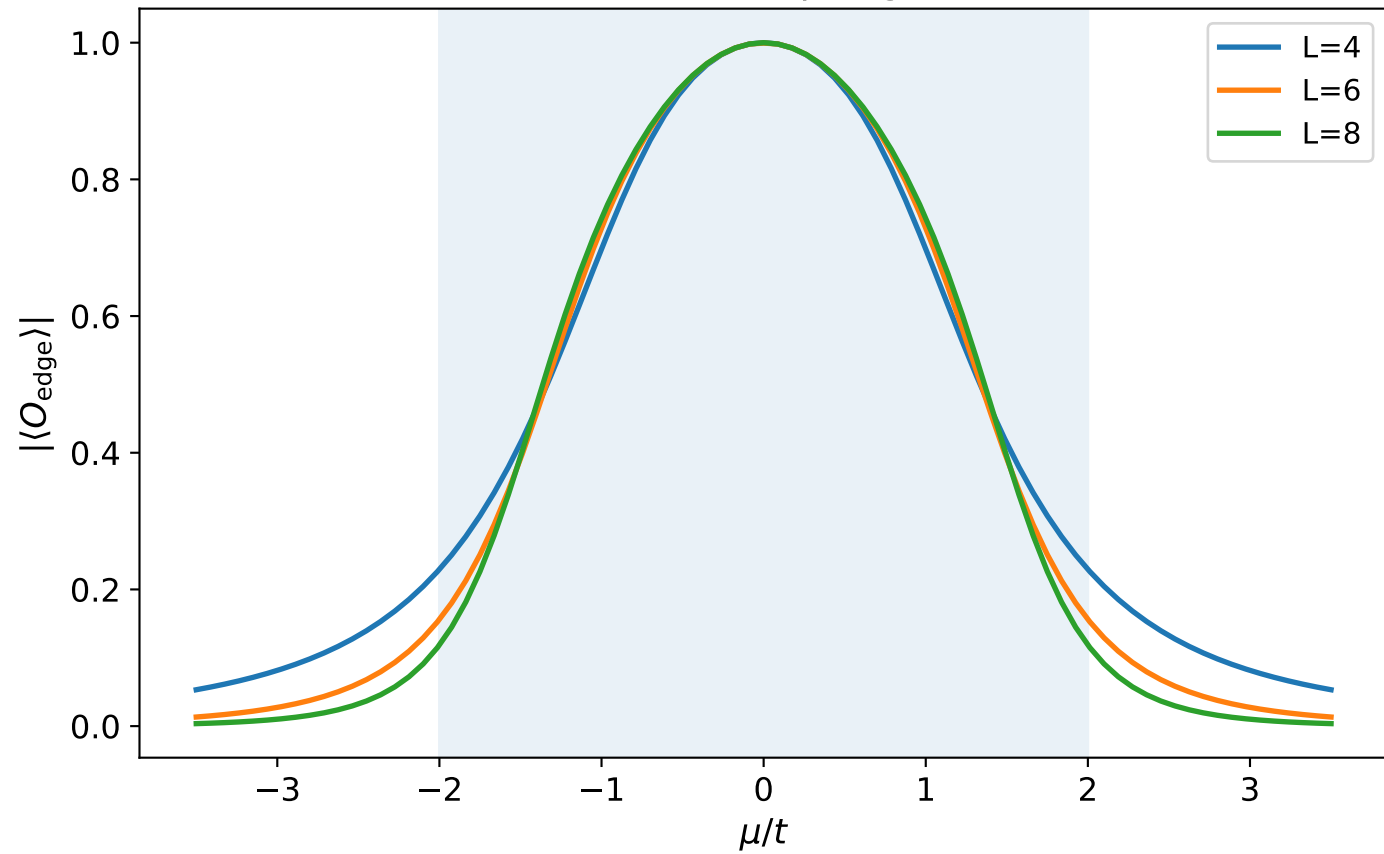
Finite-size effects on topological correlator
