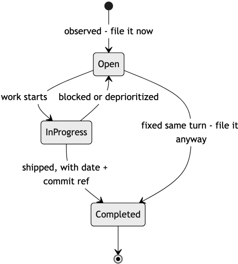
The entry state machine. Note both paths into Completed: even a same-turn fix passes through the file.
