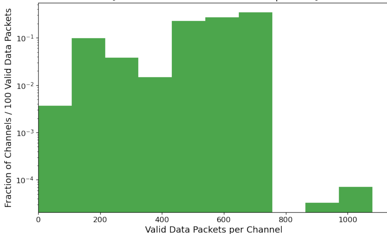
Nominal_Pedestal_Correct_Triggering Dataset on 2025_08_26 [Excludes Channels with >2000 packets]
