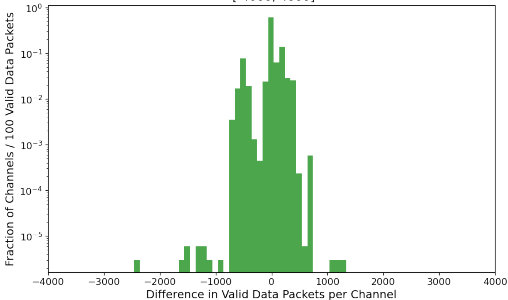
WholeDetector Dataset on 2025_08_22 MINUS Nominal_Pedestal_Correct_Triggering Dataset on 2025_08_26 [-4000, 4000]
