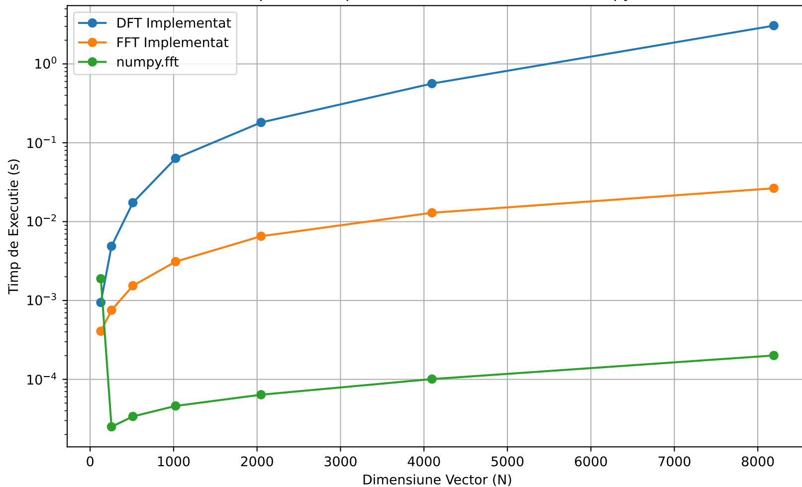
Comparare Timpi de Executie DFT vs FFT vs numpy.fft
